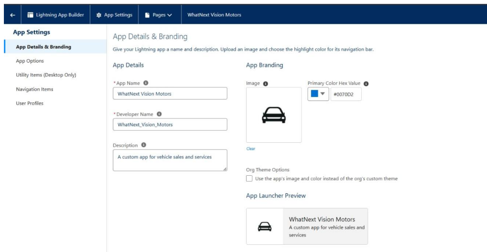
Fig 11 Lightning App
