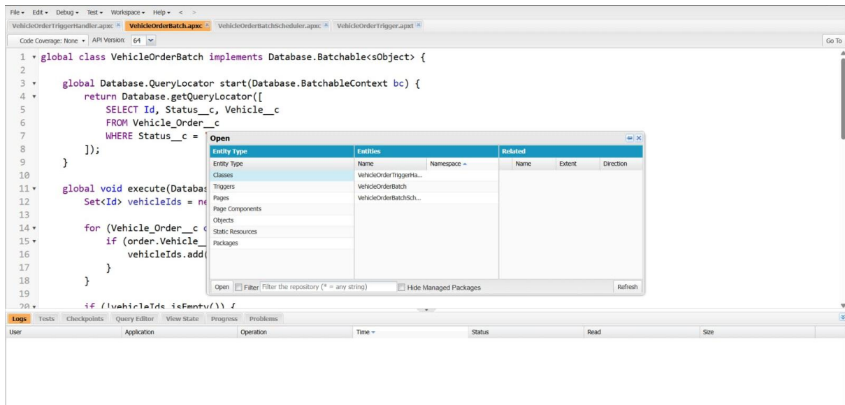
Fig 10 Apex Classes
