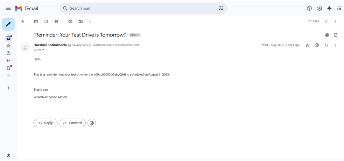
Fig 8 Reminder Mail
